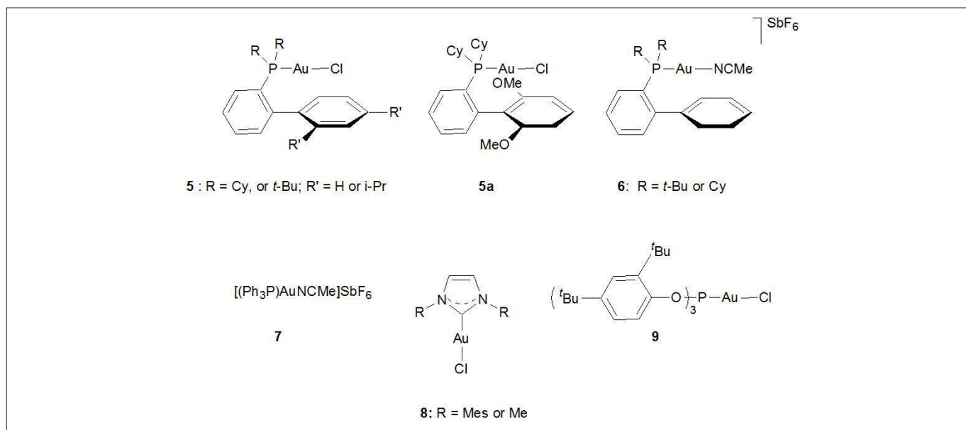
FIGURE 1: Alkynophilic gold complexes 5–8 used in [4 + 2] cycloaddition of enynes.
