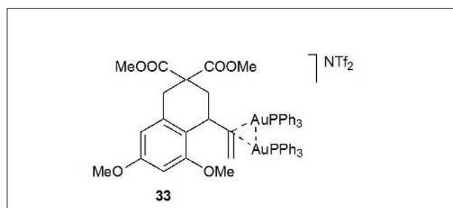
FIGURE 5: Isolated dinuclear gold complex intermediate.
