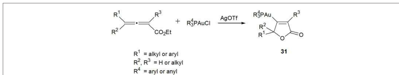
SCHEME 9: (Vinyl)gold complex 31, prepared from allenolates.
