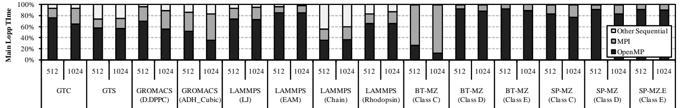
(b) On Smoky, simulations run on 512 (128 MPI proc. \times 4 OpenMP threads) and 1024 cores (256 MPI proc. \times 4 OpenMP threads).
