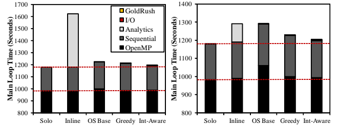
(a) w/ Parallel Coordinates (b) w/ Time Series Figure 12. GTS performance with 12288 cores on Hopper.
