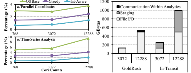
(a) Scaling of GTS Slowdown (b) Data Movement Costs Figure 13. Scaling results on Hopper. Figure 13 (a) shows the slowdown of GTS (comparing to Solo case) with different scheduling policies. Figure 13 (b) compares the data movement costs of running parallel coordinates in situ vs. in transit.
