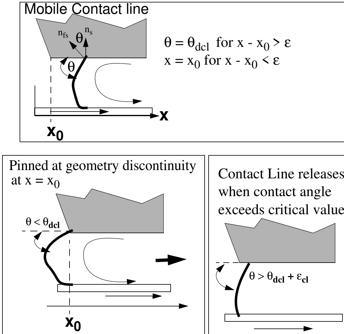
Figure 5. Contact angles and Gibbs' inequality condition in Goma, for the special case when the meniscus is moving along a surface of constant x .
