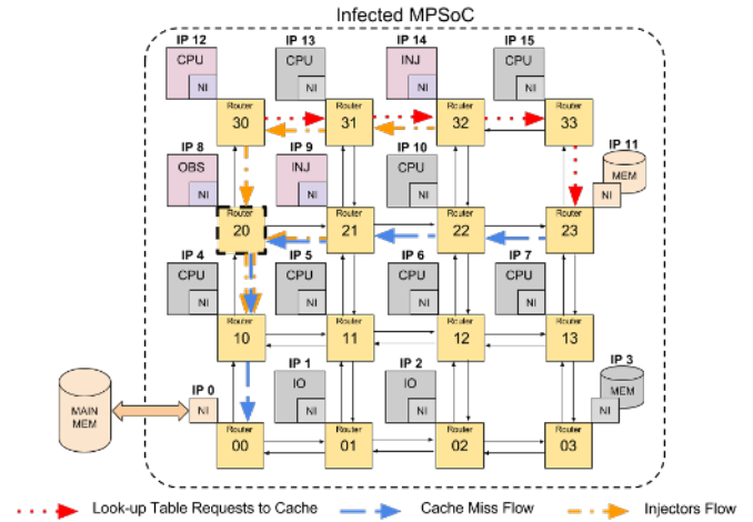
Fig. 1: MPSoC system running a sensitive application, after infection stage.
