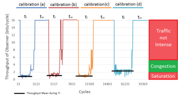
Fig. 2: Throughput Trace from observer attacker. Four calibration scenarios: a) Three injectors at 50%; b) Three injectors at 30%; c) Two injectors at 50%; d) Two injectors at 30%.
