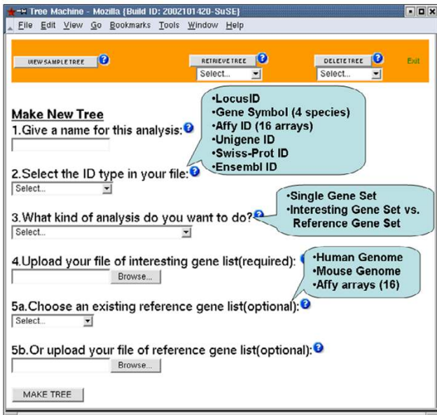
Figure 2 Input user interface of the GOTM Input interface for uploading analysis parameters (analysis name, ID type and analysis type) and data (interesting gene list and reference gene list).
