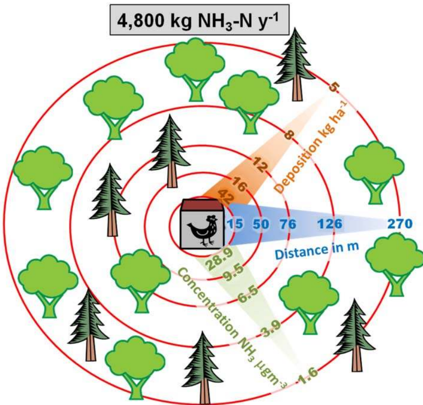
Fig. 8. Farm scale \text{NH}_3 emission and deposition, illustrating the rapid fall-off in deposition levels with distance from source (adapted from Fowler et al., 1998 and modified from version presented in Simpson et al., 2011).
