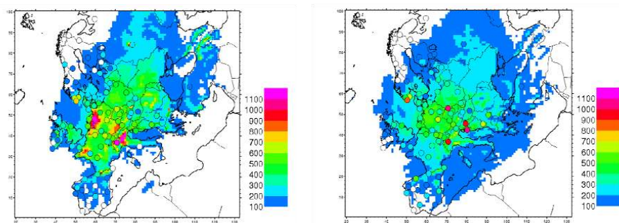
Fig. 9. Comparison of modelled and observed annual wet deposition of to the left \text{NH}_x and to the right \text{NO}_3^- ( \text{HNO}_3 and aerosol phase \text{NO}_3^- ). Data are for 2001 in the EMEP model with observations. The bullets depict observations with the same colour bas as the modelled field. Measured annual deposition is calculated by using the measured precipitation amount and the \text{NO}_3^- and \text{NH}_4^+ concentration in precipitation. Source: Simpson et al. (2011).
