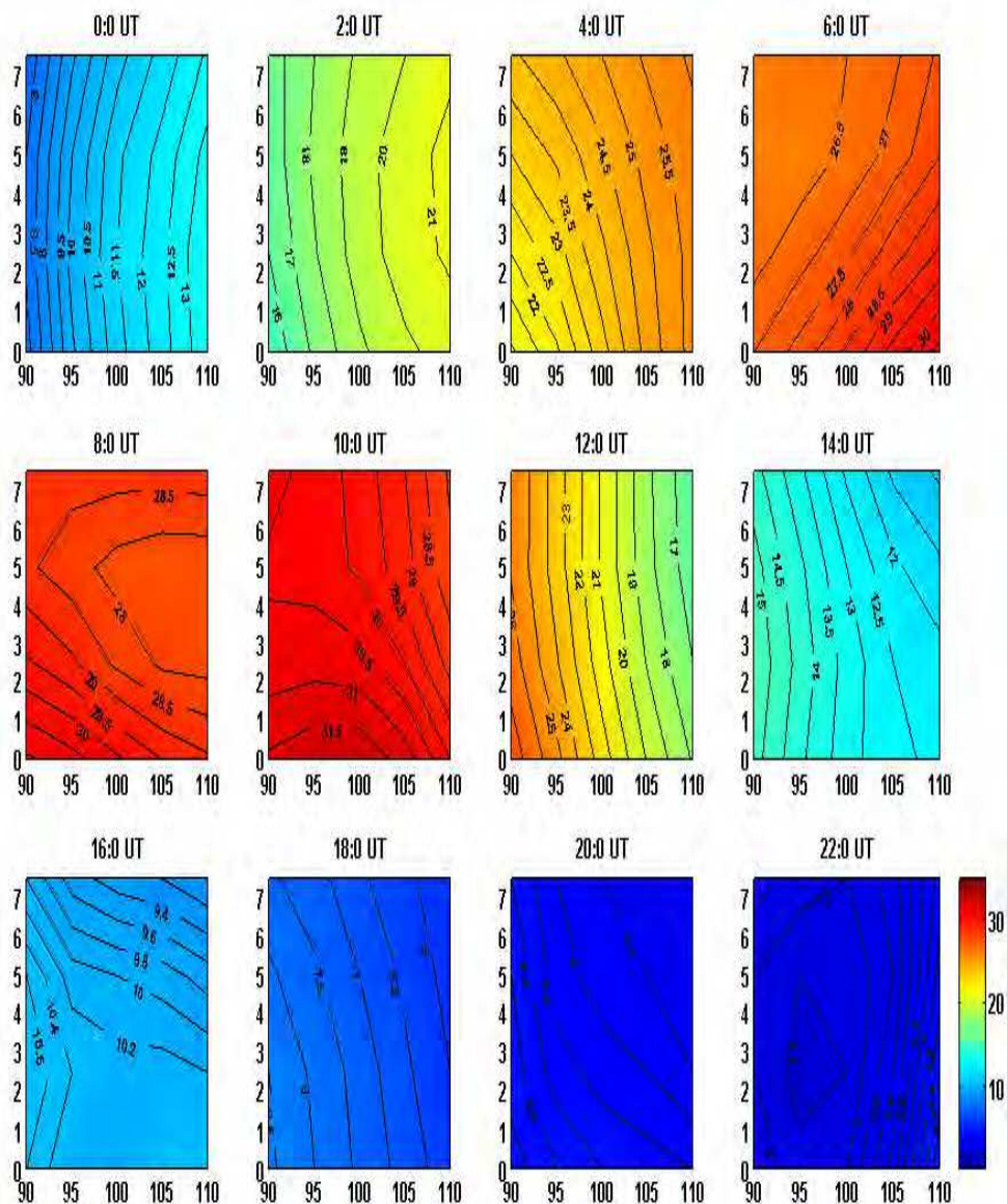
Fig. 13. TEC map from IGS, 8 November 2005
