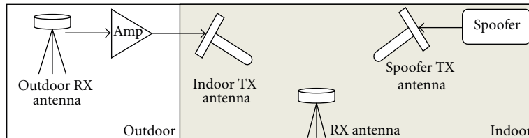
FIGURE 11: Spoofing test using GPS indoor signal retransmission.
