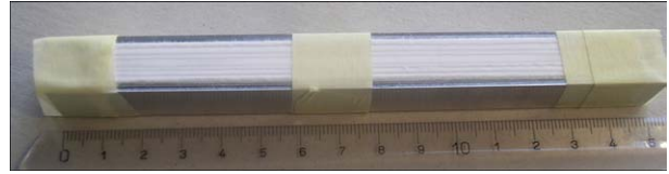
Fig. 1. A preform consisting of a stack of salt layers and aluminium sheets.
