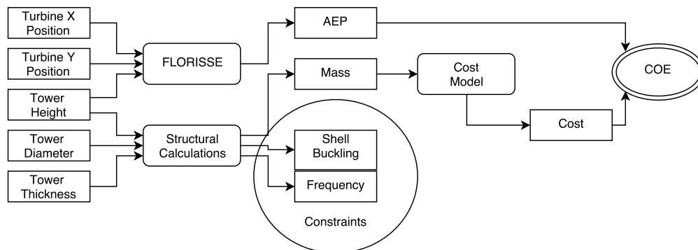
Figure 3. A simplified flow chart of COE calculation. Note that tower diameter and tower thickness are both vectors to describe the varying tower diameter and thickness along the height. The circled boxes on the bottom, shell buckling and frequency, are used as constraints in the optimization and are not used in the calculation of COE. The five boxes on the left are the design variables, and the five boxes in the middle (AEP, Mass, Shell Buckling, Frequency, and Cost) are intermediate variables.
