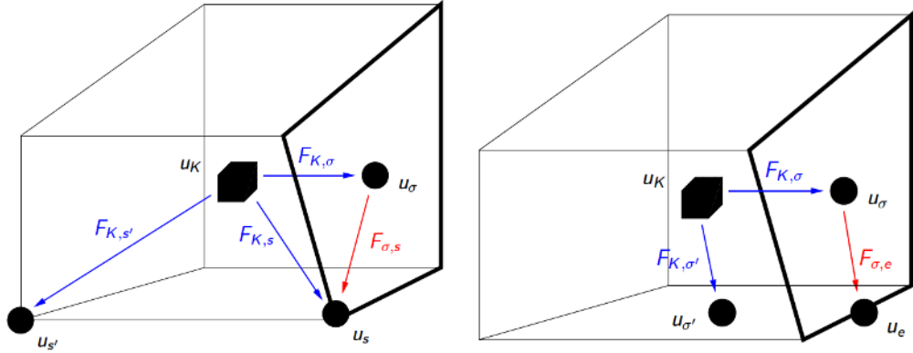
Figure 4: Matrix (in blue) and fracture (in red) fluxes inside a cell K with a fracture face \sigma (in bold) for the VAG (left) and HFV (right) schemes. The matrix fluxes F_{K,\nu} connect the cell K to the d.o.f. \nu \in dof_{\partial K} located at the boundary of K . The fracture fluxes F_{\sigma,\nu} connect the face \sigma to the d.o.f. \nu \in dof_{\partial \sigma} located at the boundary of \sigma .
