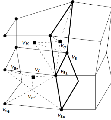
Figure 2: Degrees of freedom of the VAG scheme: cell unknowns v_K, v_L , fracture face unknown v_{\sigma} , and node unknowns v_{\mathbf{s}}, v_{\mathbf{s}_1}, v_{\mathbf{s}_2}, v_{\mathbf{s}_3}, v_{\mathbf{s}_4} . The fracture faces of \mathcal{F}_{\Gamma} are in bold. The value of v_{\sigma'} is obtained by interpolation of the node unknowns v_{\mathbf{s}_1}, v_{\mathbf{s}_2}, v_{\mathbf{s}_3}, v_{\mathbf{s}_4} of the face \sigma' \in \mathcal{F} \setminus \mathcal{F}_{\Gamma} while v_{\sigma} is kept as an unknown for \sigma \in \mathcal{F}_{\Gamma} .
