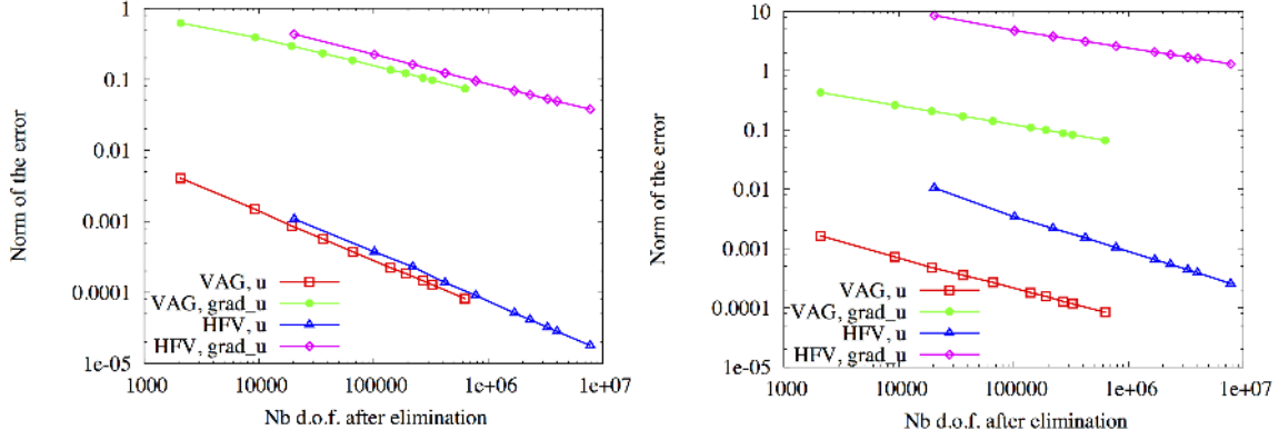
Figure 7: Second test case. For the 10 tetrahedral meshes and for the isotropic (left) and anisotropic (right) subcases: sum of L^2 norm of the relative error in the matrix and in the fracture for the function and its gradients reconstruction both for VAG and HFV schemes as the function of the number of d.o.f.(after elimination of the cell and Dirichlet unknowns).
