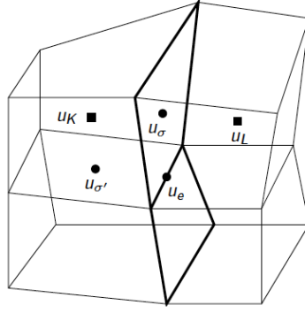
Figure 3: Degrees of freedom of the HFV scheme: cell unknowns u_K, u_L , fracture face unknown u_\sigma , matrix face unknown u_{\sigma'} and fracture edge unknown u_e .
