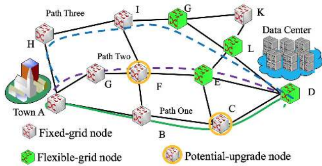
FIGURE 3. Migration scenario with traffic stability issue.
