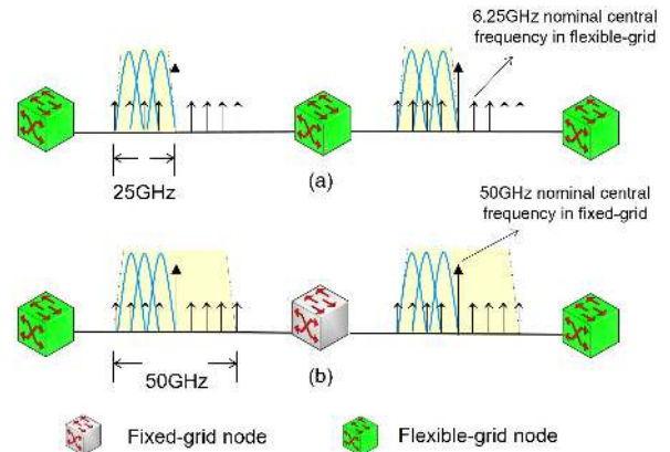
FIGURE 2. Spectrum allocation: (a) lightpath through the nodes those are all upgraded nodes; (b) lightpath goes through the fixed-grid node.
