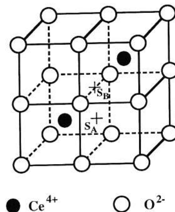
Fig. 6. Unit cell of the fluorite crystal structure.
