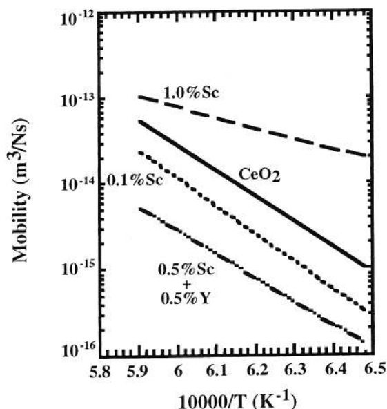
Fig. 10. Grain boundary mobility of undoped and doped CeO 2 .
