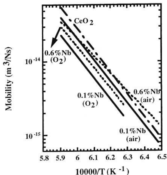
Fig. 9. Grain boundary mobility of Nb-doped CeO 2 .
