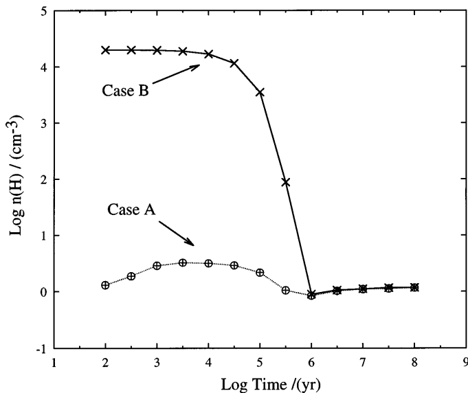
FIG. 1.—Atomic hydrogen gaseous abundance ( \text{cm}^{-3} ) in the MMs, plotted against the cloud evolutionary time for the two cases of initial atomic hydrogen abundances: case A, in which the initial form is predominantly molecular, and case B, in which the initial form is predominantly atomic.
