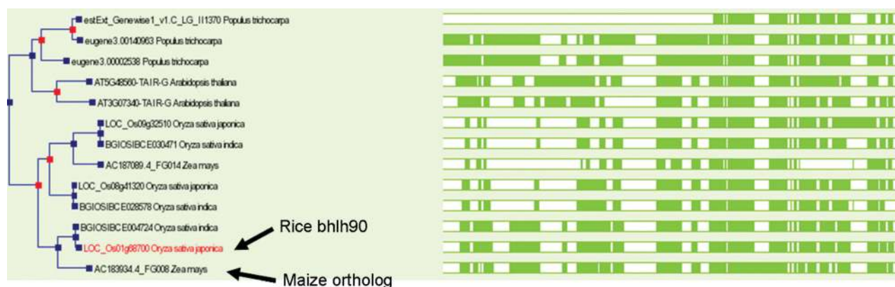
Figure 3. The rice bhlh90 gene tree (partial) showing the orthologous genes between rice, maize, A. thaliana and poplar. The full tree can be viewed at http://tinyurl.com/3clrvj . Note the bhlh90 gene is mapped in the region shown in Figure 2, but its maize gene ortholog is a predicted gene and has not been studied functionally. The solid box on the right shows the aligned regions in the proteins. It is expected that there are more maize orthologs to be identified after the maize genome sequence becomes complete.
