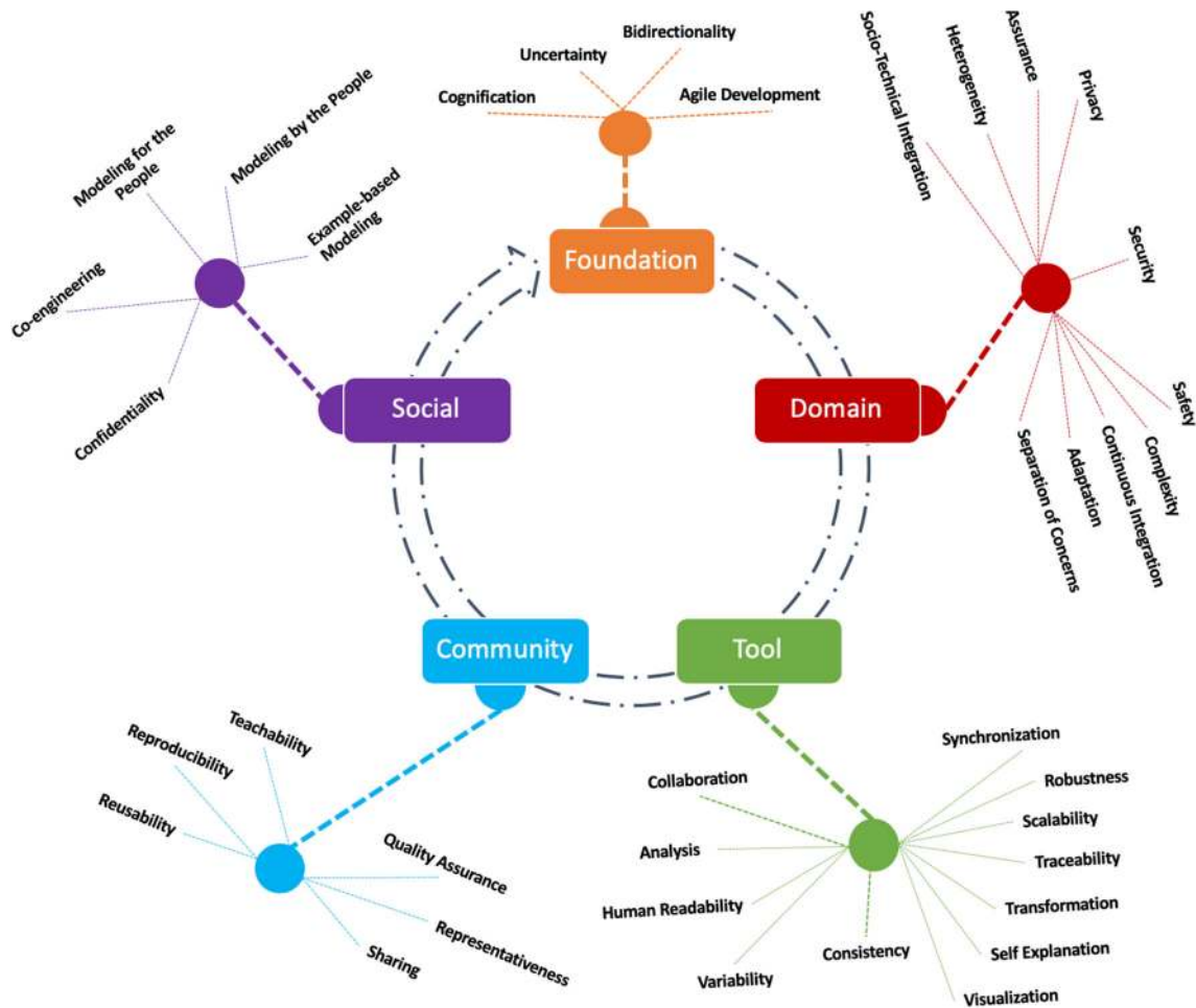
Fig. 1 Challenges classification
