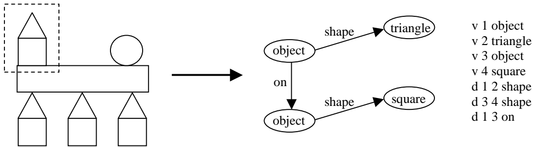
Figure 1: Example substructure in graph form with textual description. The input file syntax is v\ id\ label for vertices, d\ id1\ id2\ label for directed edges, and u\ id1\ id2\ label for undirected edges.
