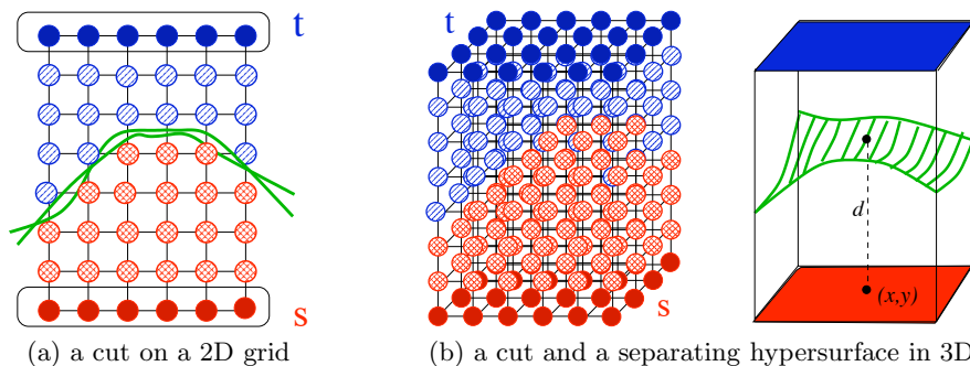
Fig. 2. s-t cut on a grid corresponds to binary partitioning of N-D space where the grid is embedded. Such space partitioning may be visualized via a separating hypersurface. As shown in (a), multiple hypersurfaces may correspond to the same cut. However, such hypersurfaces become indistinguishable as the grid gets finer.
