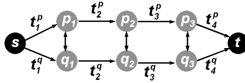
Fig. 6. Part of the graph construction for energy minimization in 3 , |\mathcal{L}| = 4
