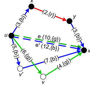
Figure 4: Multi-edge example.
