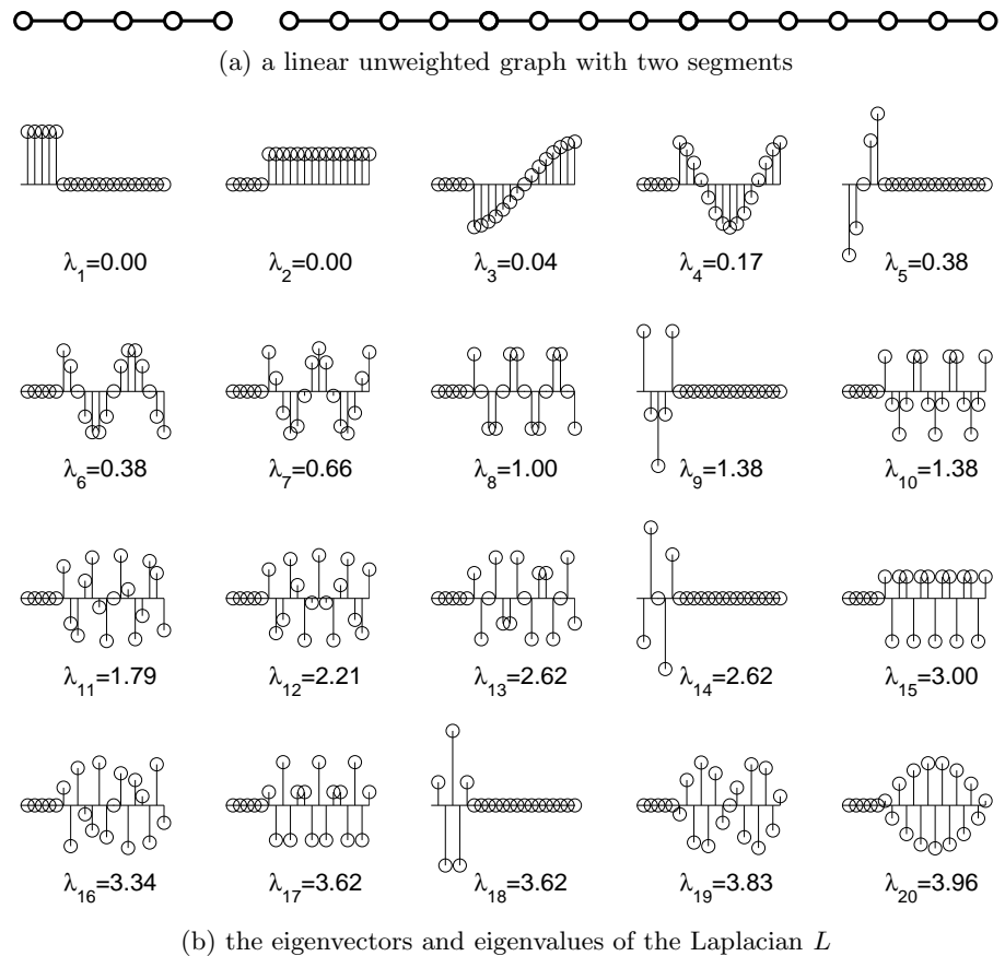
Figure 1.1 A simple graph and its Laplacian spectral decomposition. Note the eigenvectors become rougher with larger eigenvalues.
