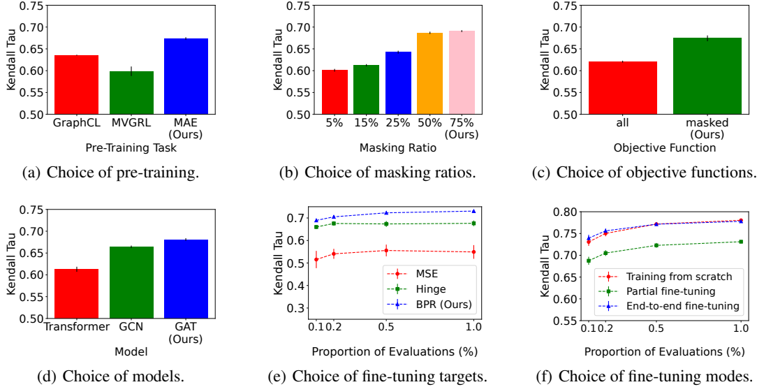
Figure 5: The ablation studies of pre-training methods, masking ratios, objective functions, models, fine-tuning targets, and fine-tuning modes, in NAS-Bench-101. It reports the mean and standard deviation of Kendall \tau of 10 independent runs.
