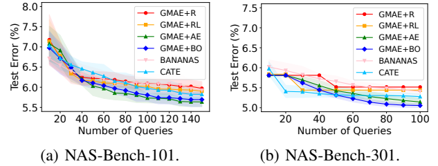
Figure 4: The comparison between GMAE-enhanced strategies and SOTA NAS methods in NAS-Bench-101 (left) and NAS-Bench-301 (right). It reports the mean and standard deviation of test error of 10 independent runs. The maximum number of queries is set to 150 for NAS-Bench-101 and 100 for NAS-Bench-301.
