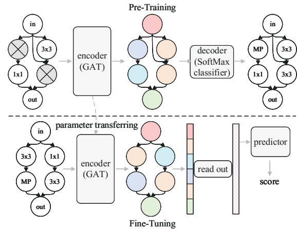
Figure 1: The overview of GMAE.
