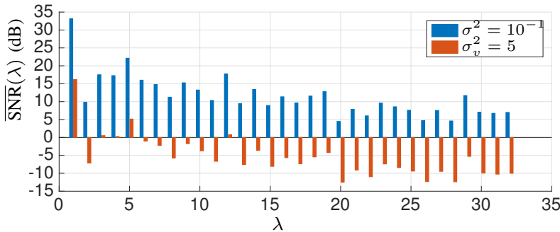
Figure 8.3: Average SNR per graph frequency for the two different noise powers computed as \overline{\text{SNR}}(\lambda_n) = \sum_{\tau=1}^{744} \hat{r}_n^2 / T \sigma_v^2 . In the high noise regime, we observe that most frequencies experience a negative SNR.
