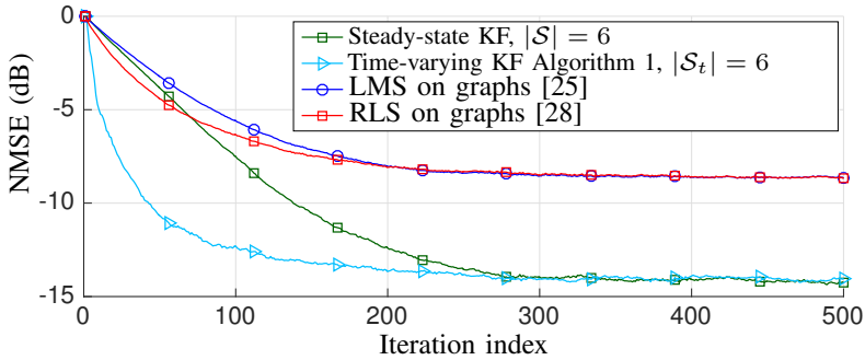
Figure 8.11: Estimated NMSE versus iteration index for steady-state KF ( |\mathcal{S}| = 6 chosen with Algorithm 8.2), time-varying KF ( |\mathcal{S}_t| = |\mathcal{S}| = 6 chosen randomly for each iteration), as well as RLS ( \beta_{\text{RLS}} = 0.99 ) and LMS ( \mu_{\text{LMS}} = 0.041 ) with maximum sampling rate |\mathcal{S}_t| = |\mathcal{F}| = 18 .
