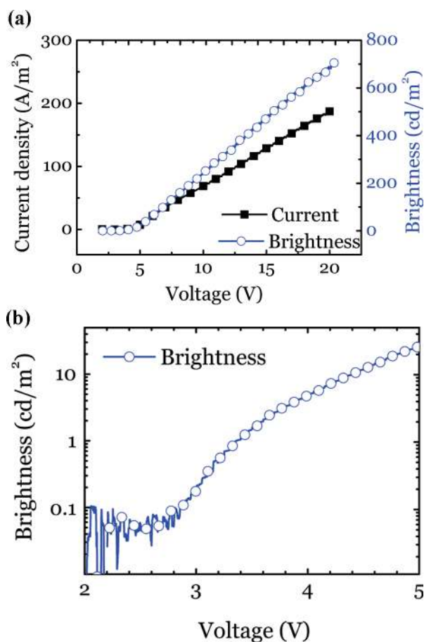
Figure 2. Optoelectronic performance of a carbon-based, metal-free LEC. Current density (solid black squares) and brightness (open blue circles) as a function of voltage for a PEDOT-PSS/(SY+PEO+ \text{KCF}_3\text{SO}_3 )/graphene device, recorded at a scan rate of 0.01 V/s. (a) Brightness as a function of voltage in linear scale. (b) shows the same plot as (a) but in logarithmic scale near the turn-on voltage.
