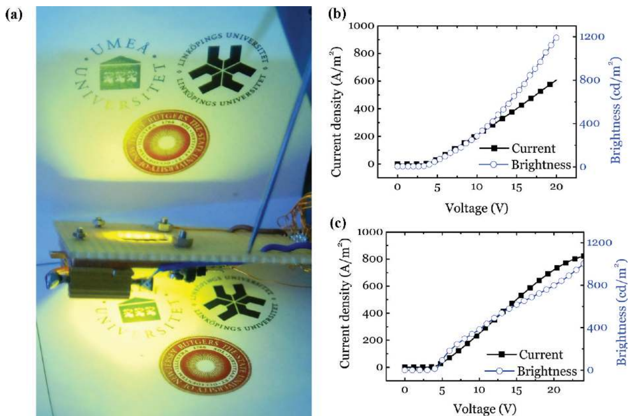
Figure 3. Omni-directional light emission from a carbon-based, metal-free LEC. (a) Photograph of the two-sided emission from the sandwich device. The edge of the light-emitting device is visible in the specially designed holder. Light coming through the PEDOT-PSS anode illuminates a sheet of paper above the device, while the light visible from the lower side of the device has passed through the graphene cathode. (b) Current density and brightness, measured through the graphene cathode, versus applied potential swept at 0.1 V/s. (c) Current density and brightness, measured through the PEDOT-PSS anode at the same sweep rate. University logos used with permission from Linköping University, Umeå University, and Rutgers University.
