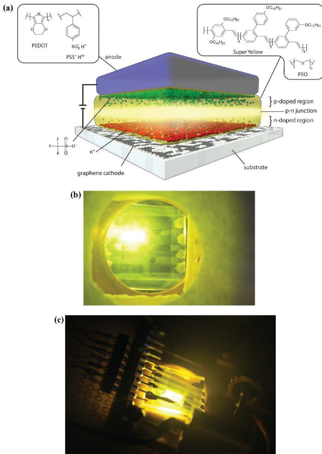
Figure 1. All-plastic, solution-processed LECs. (a) Schematic illustrating the structure and operation of the device. During operation, light is emitted both upward, through the PEDOT-PSS electrode, and downward, through the graphene electrode. (b) Photograph of an LEC during light emission, as viewed through the graphene cathode. (c) Similar photograph, as viewed through the PEDOT-PSS anode. Photo courtesy of the authors.
