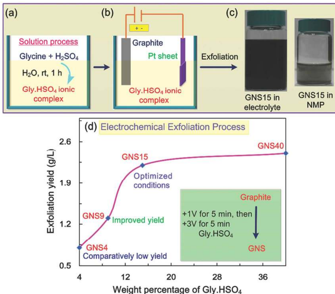
Fig. 3. Preparation process of graphene. (a) A simple solution-process approach for Gly· \text{HSO}_4 ionic complex preparation in aqueous solution. (b) Diagram of electrochemical experimental setup. (c) Photographs of graphene directly in electrolyte (left) and re-dispersed in NMP after purification (right). (d) Exfoliation yields versus weight ratios of Gly· \text{HSO}_4 ionic complex to water used in exfoliation experiments. Copyrights reserved to the John Wiley and Sons. 86
