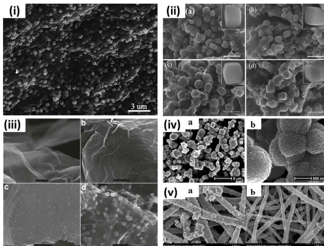
Fig. 18. SEM images of various HRG/TiO 2 nanocomposites. (i) As-prepared HRG/TiO 2 nanocomposites synthesized via hydrothermal reaction with aqueous solutions containing (NH 4 ) 2 TiF 6 (0.03 M) and GO at 160 °C for 4 h. (ii) Illustrates the gradual change of the morphology of TiO 2 NPs with the increase of time (ii-a) cuboid-like morphology of the anatase TiO 2 NPs obtained in 2h reaction time. (ii-b) after 8 hrs, the NPs grow fatter and the four lateral facets of the cuboid-like particles rose in the waist. (ii-c) after 12 hrs (ii-d) after 24 h, the NPs turned into truncated octahedral morphologies. The inset shows the corresponding magnified SEM images. Copyrights reserved to the RSC publishing. 437 (iii) SEM images of HRG treated in the sulfuric acid reaction solution containing titanium sulfate at 100 C (a) pristine graphene sheets (b) after 1 h (c) after 4 h (d) after 6 h. scale bar in (a-d) 400 nm. Copyrights reserved to the John Wiley & Sons, Inc. 220 (iva-b) SEM images of pristine TiO 2 . Copyrights reserved to the Elsevier Ltd. 441 (v) SEM images of (a) TiO 2 -CNF (carbon nanofibers) (b) TiO 2 -CCNF (Carbon composite nano fibers). Copyrights reserved to the Elsevier Ltd. 442
