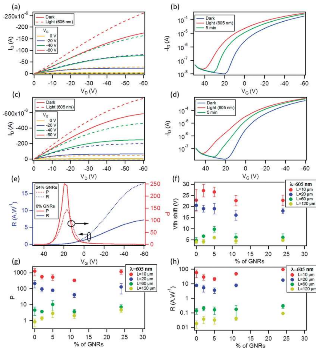
Fig. 8 Comparison of (a) output and (b) transfer characteristics at V_D = -60 V of a device with 24% GNR blend with the same channel length L = 20 \mu\text{m} measured in the dark and under monochromatic light ( \lambda = 605 nm; 8.17 \text{mW cm}^{-2} ). (c) output and (d) transfer characteristics at V_D = -60 V of a device with 24% GNR blend with the same channel length L = 20 \mu\text{m} measured in the dark and under monochromatic light ( \lambda = 605 nm; 8.17 \text{mW cm}^{-2} ). (e) Variation of the responsivity R (blue curves) and photosensitivity P (red curves) with V_G at V_D = -60 V at \lambda = 605 nm for OFETs ( L = 20 \mu\text{m} ) with 0% (solid lines) and 24% blends of GNRs (dashed lines). (f) Threshold voltage shift under illumination with monochromatic light ( \lambda = 605 nm; 8.17 \text{mW cm}^{-2} ) for 4 channel length ( L = 10, 20, 60 and 120 \mu\text{m} ) OFETs based on different blend percentages of GNRs with respect to P3HT. (g) Photosensitivity (extracted at V_G = 20 V), and (h) responsivity of these devices (extracted at V_G = -60 V) both at V_D = -60 V. The left axis is expressed in log-scale.
