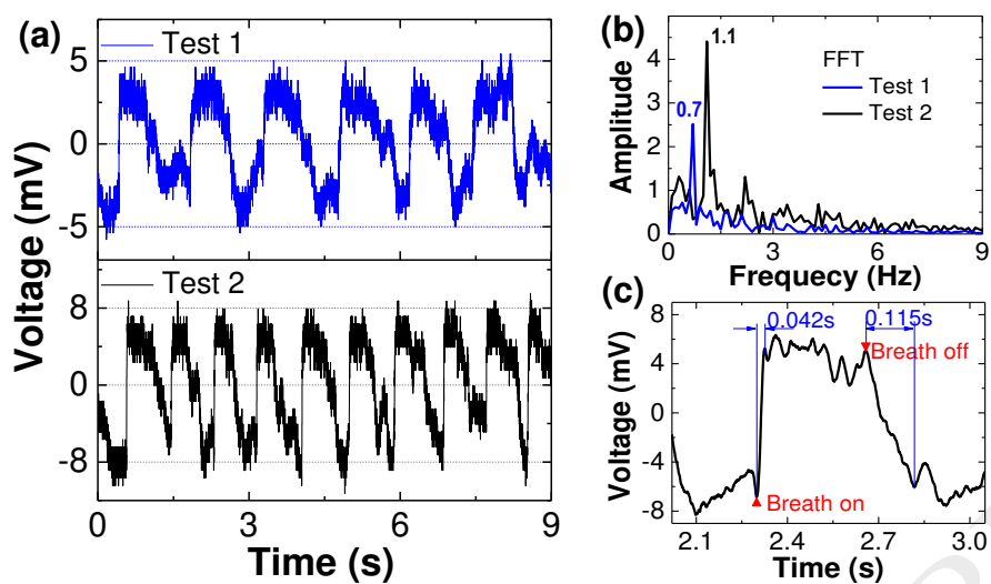
Fig. 7. (a) Responses of GO-deposited TFG to human breathing, including normal (top) and rapid (bottom) breathing, and (b) their FFT results, displaying different breathing frequencies. (c) Enlarged view of the temporal waveform to evaluate the response and recovery time.
