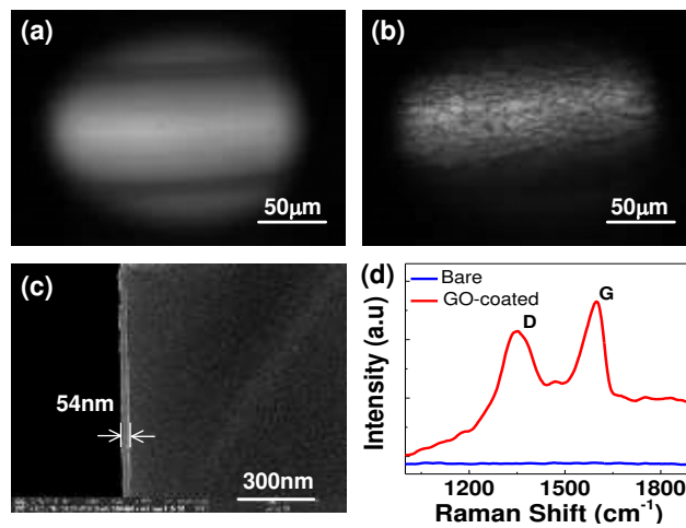
Fig. 4. Optical microscope images of (a) bare and GO-coated TFG at the magnification of 60 \times , (c) SEM image of the zoomed cross section of the GO-coated TFG, and (d) Raman spectra of bare and GO-coated TFG showing the G and D bands of GO.
