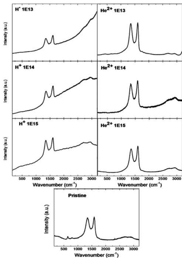
Fig. 6 The Raman spectra of pristine and irradiated GO foils. The ion beam irradiation was performed using 2.5 MeV \text{H}^+ and 5.1 MeV \text{He}^{2+} ions with different ion irradiation fluencies.
