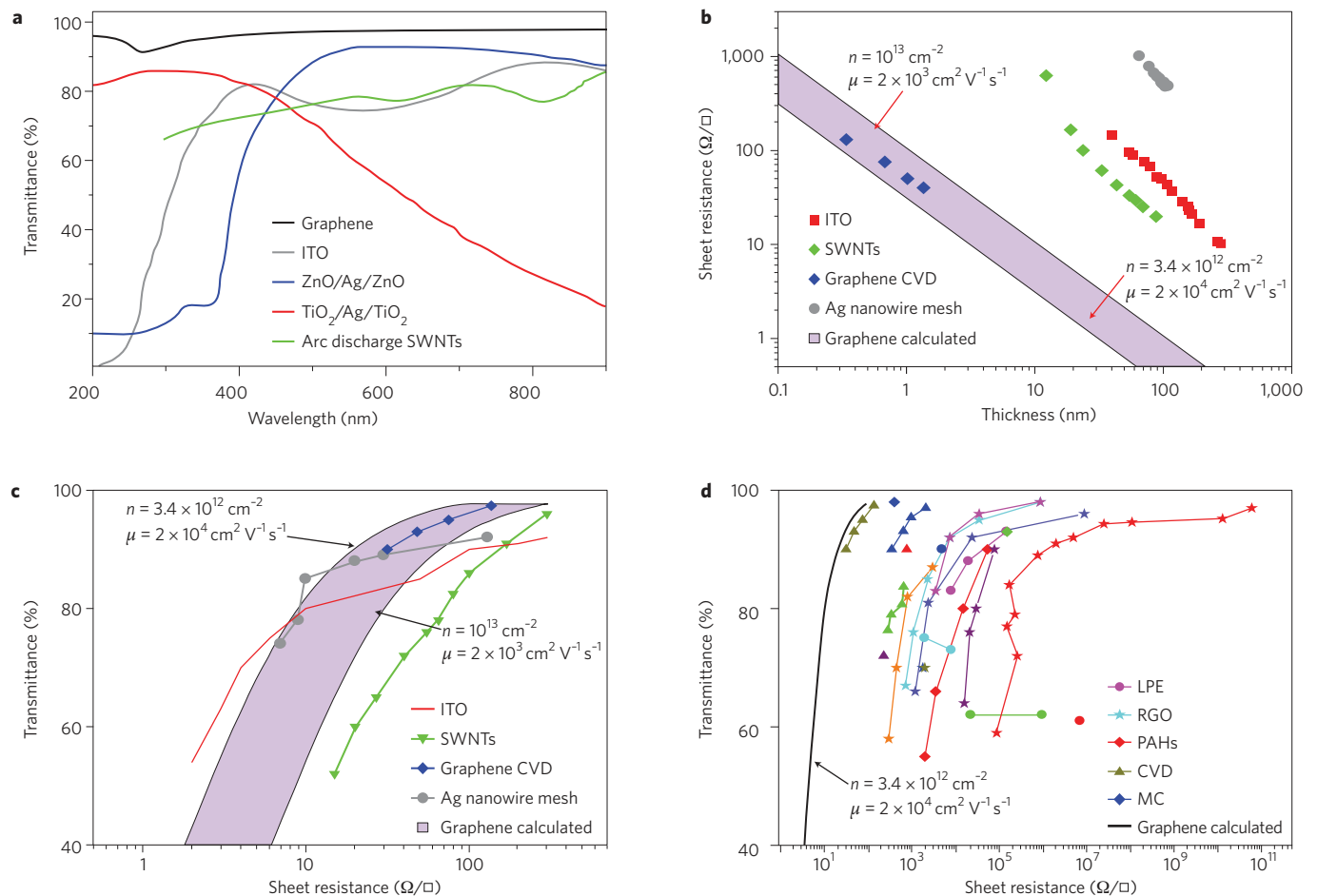
Figure 2 | Graphene as transparent conductor. a , Transmittance for different transparent conductors: GTCFs 39 , single-walled carbon nanotubes (SWNTs) 77 , ITO 75 , ZnO/Ag/ZnO (ref. 81) and TiO 2 /Ag/TiO 2 (ref. 70). b , Thickness dependence of the sheet resistance. The blue rhombuses show roll-to-roll GTCFs based on CVD-grown graphene 39 ; red squares, ITO 75 ; grey dots, metal nanowires 75 ; green rhombuses, SWNTs 77 . Two limiting lines for GTCFs are also plotted (enclosing the shaded area), calculated from equation (6) using typical values for n and \mu . c , Transmittance versus sheet resistance for different transparent conductors: blue rhombuses, roll-to-roll GTCFs based on CVD-grown graphene 39 ; red line, ITO 75 ; grey dots, metal nanowires 75 ; green triangles, SWNTs 77 . Shaded area enclosed by limiting lines for GTCFs calculated using n and \mu as in b . d , Transmittance versus sheet resistance for GTCFs grouped according to production strategies: triangles, CVD 37–39,97 ; blue rhombuses, micromechanical cleavage (MC) 88 ; red rhombuses, organic synthesis from polyaromatic hydrocarbons (PAHs) 65 ; dots, liquid-phase exfoliation (LPE) of pristine graphene 44,45,48,88 ; and stars, reduced graphene oxide (RGO) 52,54,83,84,96 . A theoretical line as for equation (6) is also plotted for comparison.
