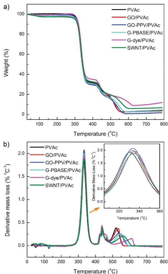
Figure 7. a) TGA and b) DTG analyses of PVAc and four types of graphene-based and SWNT-based polymer nanocomposites. The inset in b shows the enlarged DTG peak at \sim 330^\circ\text{C} .
