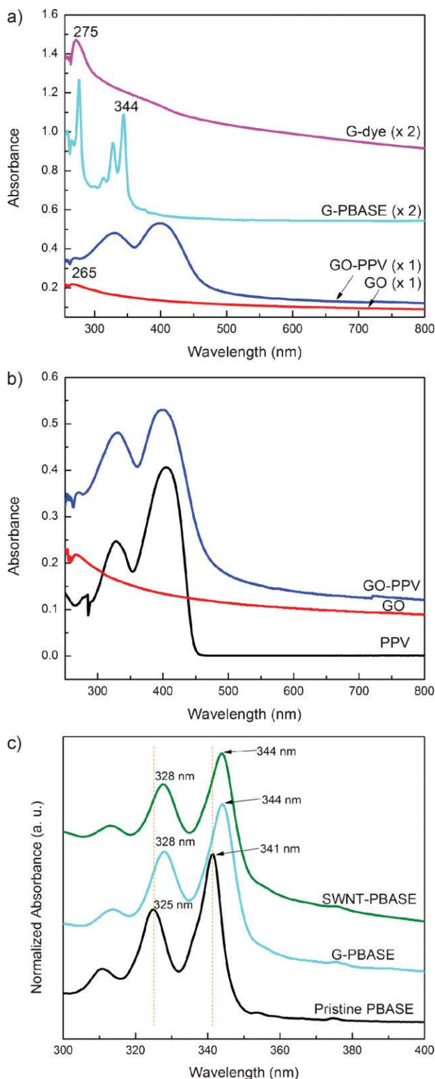
Figure 3. a) UV-vis absorption spectra of graphene derivatives. All the spectra were recorded in DMF with the same concentration ( 0.05 \text{ mg mL}^{-1} ). b) UV-vis absorption spectra of GO, PPV, and GO-PPV. c) Normalized UV-vis absorption spectra of pristine PBASE, G-PBASE and SWNT-PBASE. The spectra of G-PBASE and SWNT-PBASE have been offset for better view.
