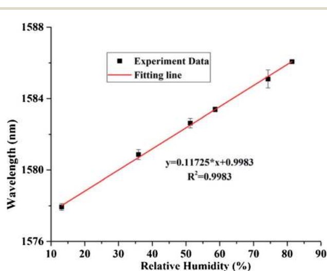
Fig. 14 Fitting line between the resonance spectrum and RH values. Reproduced with permission from ref. 148, copyright 2019, Elsevier.
