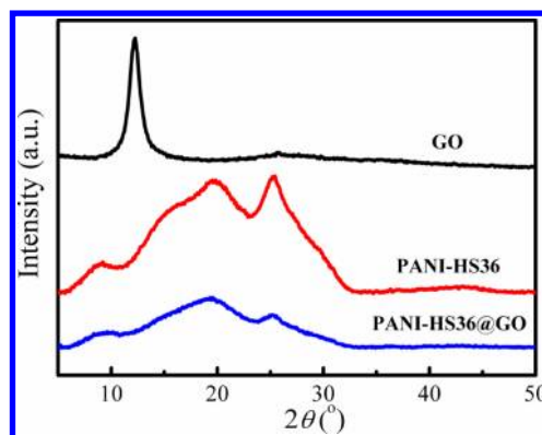
Figure 3. XRD patterns of GO, PANI-HS36, and PANI-HS36@GO hybrids.
