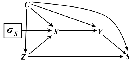
FIG. 24. Graphical representation of assumption in time-to-pregnancy example.
