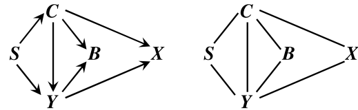
FIG. 5. Representing the sampling order: DAG (left) with moral graph on \text{An}(B \cup X \cup C \cup Y) (right).
