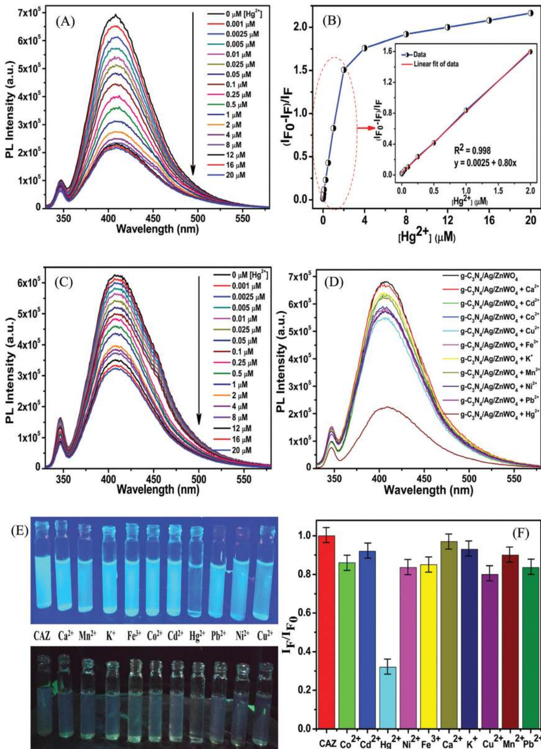
Fig. 7 (A) and (C) PL intensity responses of g-C 3 N 4 /Ag/ZnWO 4 in phosphate buffer (pH = 7.2) and tap water, respectively on the addition of different amounts of Hg 2+ , \lambda_{\text{ex}} = 310 nm, (B) calibration curve of g-C 3 N 4 /Ag/ZnWO 4 for the detection of Hg 2+ (inset is a linear plot of relative intensity vs. conc. of Hg 2+ ), (D) PL emission of g-C 3 N 4 /Ag/ZnWO 4 in the presence of different metal ions individually ( \lambda_{\text{ex}} = 310 nm, [M n+ ] = 10 μM), (E) photographic image of g-C 3 N 4 /Ag/ZnWO 4 in phosphate buffer under 365 nm light (upper panel) and white light in the presence of different metal ions (10 μM) (lower panel), and (F) bar diagram of the relative PL emission intensities ( I_F/I_{F0} ) of g-C 3 N 4 /Ag/ZnWO 4 in the presence of various metal ions (10 μM).
