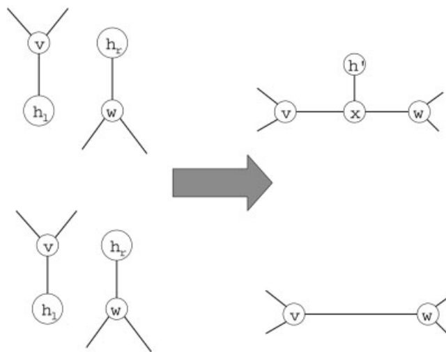
FIG. 3. Joining surjection branch decompositions.
