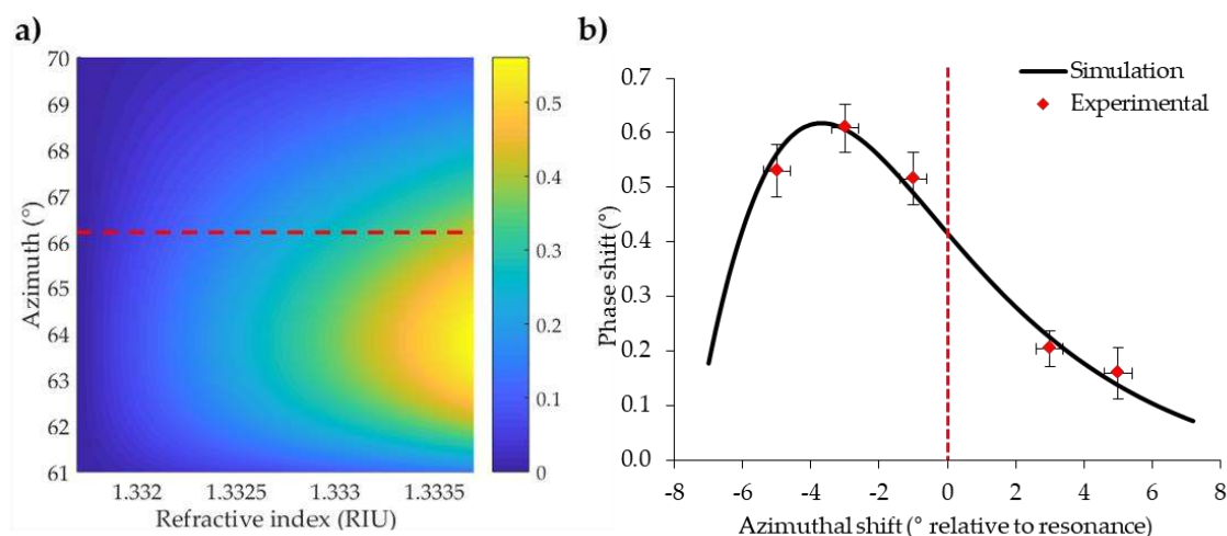
Figure 4. Numerical simulations and experimental results of azimuthal contribution to phase shift enhancement. (a) Simulated phase variation colour map of a grating with a period of 400 nm and 633 nm incident wavelength. The polar angle was fixed at 60°, while the azimuth was varied around resonance. The phase variation was simulated for a set of refractive indexes starting from the water. The dotted red line represents the resonant azimuth for water. (b) Experimental phase shift for a 200 mM NaCl solution from water (considered as reference), overlapped to the simulated longitudinal section profile from the colour map for different azimuths around resonance, at 60° polar angle. The dotted red line represents the resonant azimuth for water.
