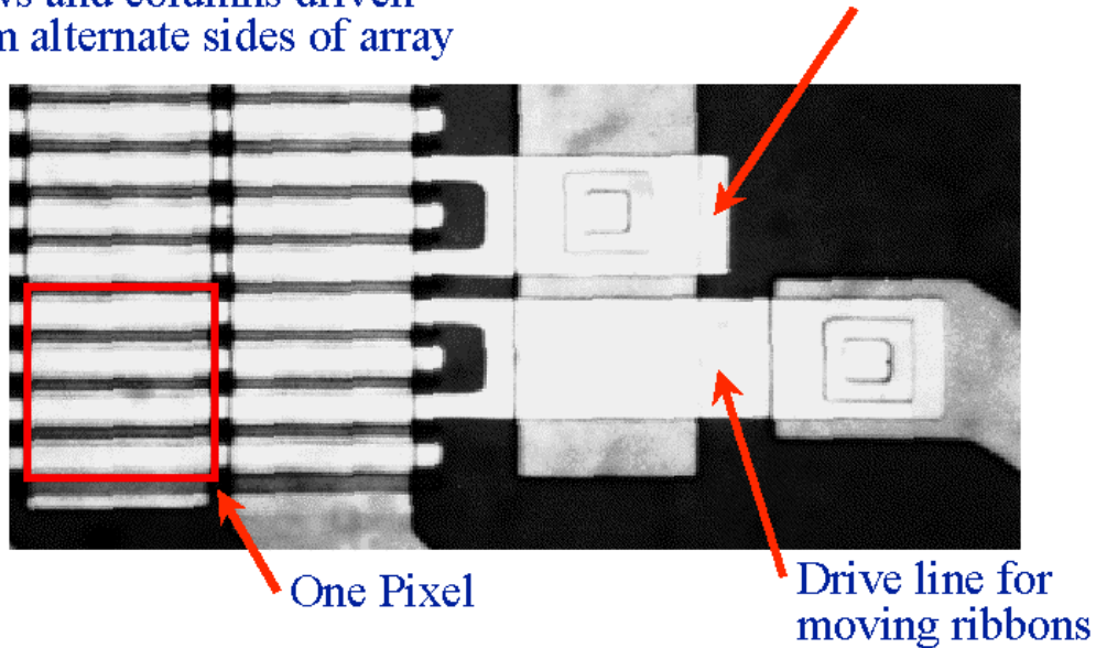
Figure 3: A single pixel consists of a pair of fixed and a pair of movable ribbons.
