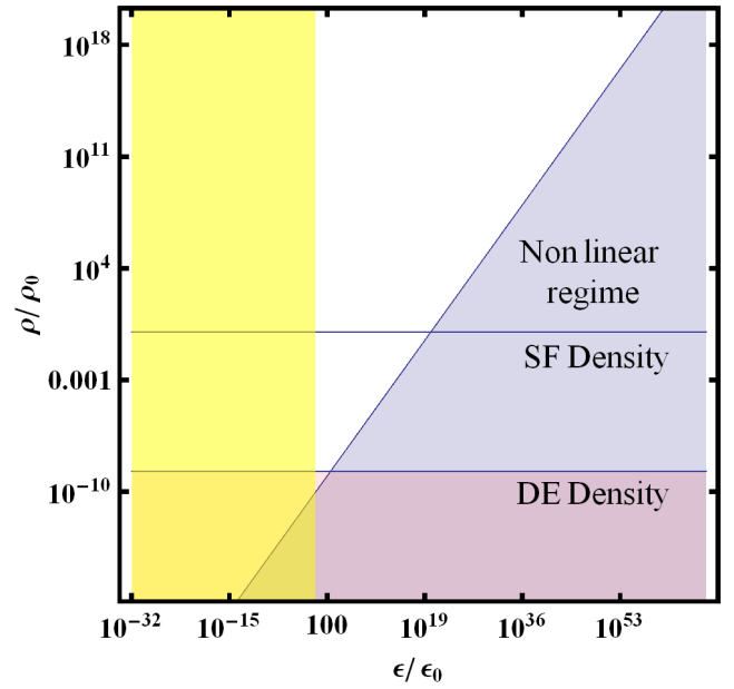
Figure 4: Analogous to Figure 2 for model 2. The limit of the region depicted in yellow shows the proposed value \varepsilon = -\mu^4 , and \mu = 10^{-42} GeV according to [27].
