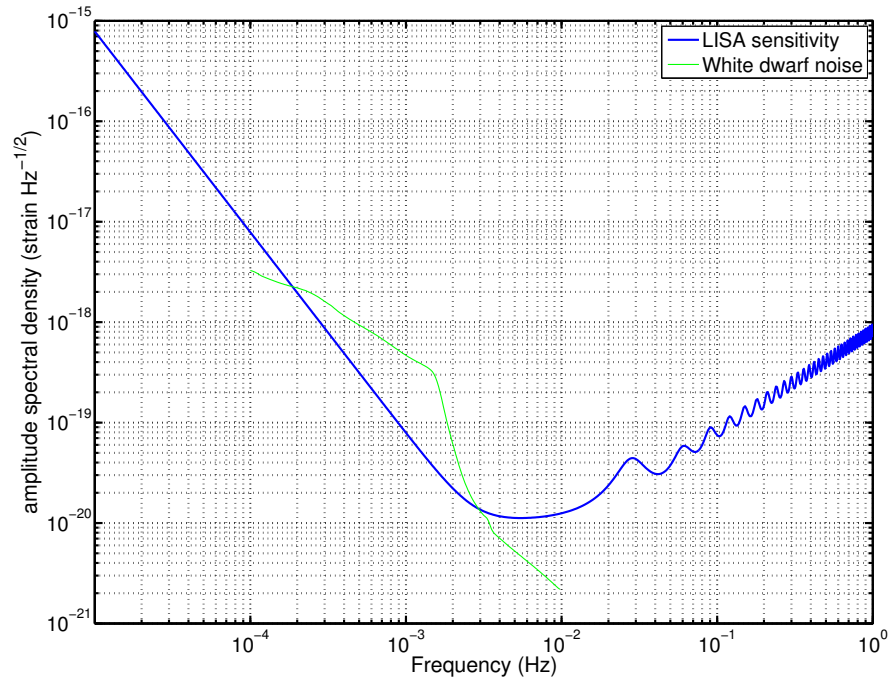
Figure 20: A design sensitivity amplitude spectral density curve for LISA created using the standard parameters in the online generator at [208]. The curve assumes equal length arms, sensitivity averaged over the whole sky and all polarisations, and an SNR of 1. Also included is a curve showing the expected background noise from galactic white-dwarf-binary systems, which will dominate over the instrumental noise in the range from \approx 0.1 - 1 mHz.
