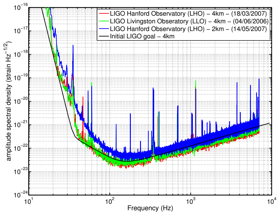
Figure 4: Measured sensitivity of the initial LIGO interferometers during the S5 science run (see Section 6.1.2). Reproduced with permission from [213].
