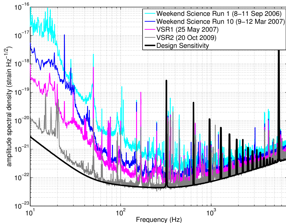
Figure 17: The best strain sensitivities from the Virgo weekend and full time science runs WSR1, WSR10, VSR1 and VSR2 [305, 57].
