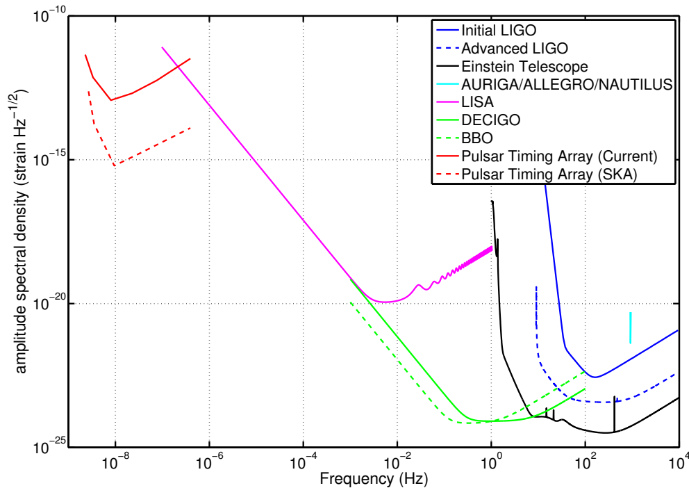
Figure 1: The sensitivity of various gravitational-wave detection techniques across 13 orders of magnitude in frequency. At the low frequency end the sensitivity detection curves for pulsar timing arrays (based on current observations and future observations with the Square Kilometre Array [108]) are extrapolated from Figure 4 in [325]. In the mid-range LISA, DECIGO and BBO are described in more detail in Section 7, with the DECIGO and BBO sensitivity curves taken from models given in [323]. At the high frequency the sensitivities are represented by three generations of laser interferometers: LIGO, Advanced LIGO and the Einstein Telescope (see Sections 6, 6.3.1 and 6.3.2). Also included is a representative sensitivity for the AURIGA [88], Allegro [226] and Nautilus [239] bar detectors.
