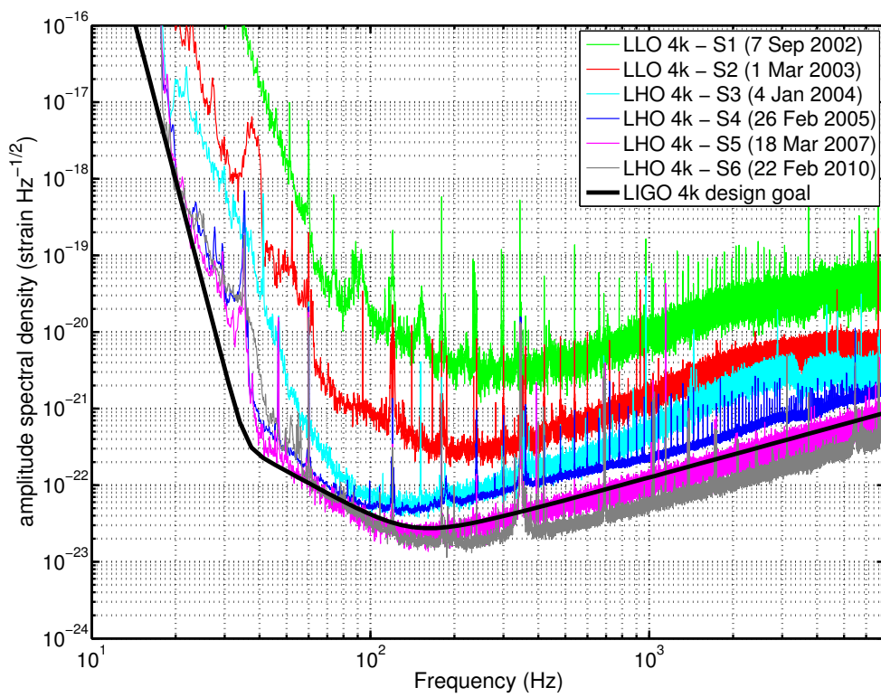
Figure 15: The best strain sensitivities from the LIGO science runs S1 through S6 [213]. The S6 curve is preliminary and based on h(t) data that has not been completely reviewed and may be subject to change. Also shown is the LIGO 4 km design sensitivity.
