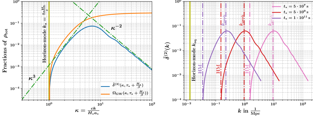
Figure 6: Left: In blue the numerical solution of Eq. (129) at the end of the phase transition and with initial conditions \tilde{\delta}^{(2)}(\kappa, t) = \tilde{\delta}^{(2)\prime}(\kappa, t) = 0 and for \alpha \rightarrow \infty and \beta/H_* = 1 . We also show the source term in orange at the end of the phase transition \tau_{\text{ev}} = \tau_* + H_*/\beta . Right: Induced density perturbation by GWs from FPT. For demonstration purposes we chose \alpha \rightarrow \infty, \beta = H_* . Shown are solutions for different scales a_* H_* in comparison with the horizon at matter-radiation equality.
