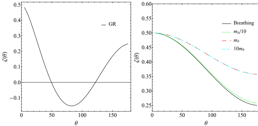
Figure 2. The normalized correlation function \zeta(\theta) = C(\theta)/C(0) as a function of \theta for the massless field \tilde{h}_{\mu\nu} (the left panel) and the scalar field \varphi (the right panel).
