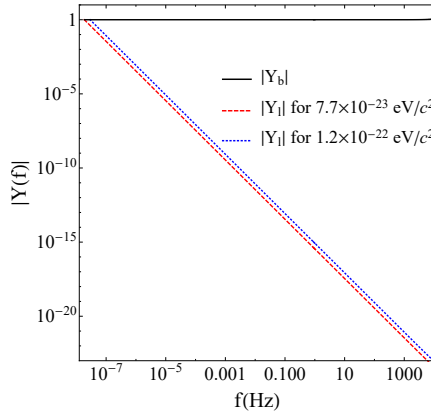
Figure 1. The absolute values of the longitudinal and transverse response functions |Y_l(f)| and |Y_b(f)| as functions of f for aLIGO to a scalar gravitational wave with the masses 1.2 \times 10^{-22} \text{ eV}/c^2 [1] (dotted blue curve) and 7.7 \times 10^{-23} \text{ eV}/c^2 [3] (dashed red curve). The solid curve denotes |Y_b(f)| .
