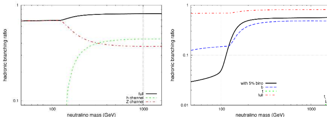
Figure 5. Left Panel: Branching ratio into a quark pair and a gravitino for a Higgsino neutralino in the limit of heavy Higgs decoupling and a SM-like light Higgs. We have taken here m_h = 115 GeV and negligible gravitino mass in the phase space factor. Right Panel: As the left panel, but showing the b\bar{b} and t\bar{t} channels and the total hadronic branching ratio with a 5% Bino fraction. Below the opening of the intermediate Z/Higgs channel, a small Bino fraction can reduce the hadronic branching ratio very effectively.
