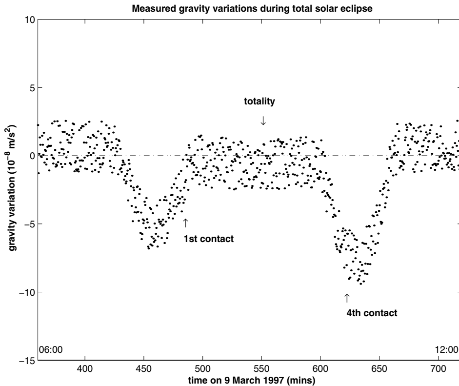
Figure 1. Measured gravity variations during the Mohe solar eclipse.
