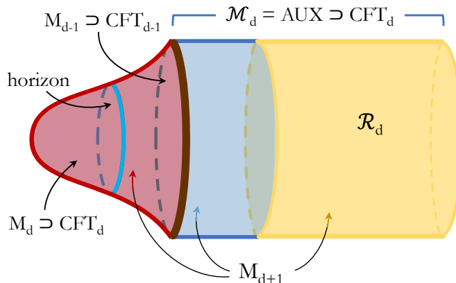
Figure 10. A doubly holographic CFT_{d-1} on M_{d-1} is coupled to holographic bath: a CFT_d on \mathcal{M}_d . The first holographic dual is M_d \cup \mathcal{M}_d , where M_d contains the same CFT_d coupled to gravity. The second holographic dual is M_{d+1} (solid interior). We consider a state which, in the first dual, corresponds to an evaporating black hole in M_d with radiation escaping to \mathcal{M}_d . The von Neumann entropy of the radiation in the subregion \mathcal{R}_d \subset \mathcal{M}_d can be computed using the single or double RT prescription.
