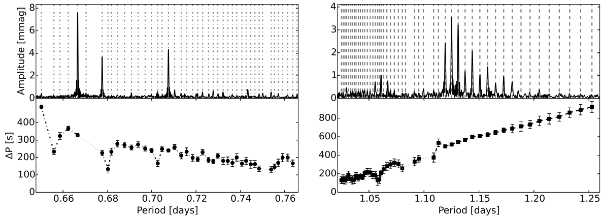
Fig. 13.— The period spacing patterns of KIC 3448365.
