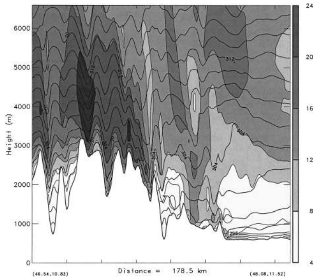
FIG. 14. Vertical sections of the v component of the wind (grayscale, interval = 4 \text{ m s}^{-1} ), located approximately along the first transverse, valid at 0630 UTC 21 Oct 1999, derived from the fourth grid mesh of COAMPS real-data simulation.
