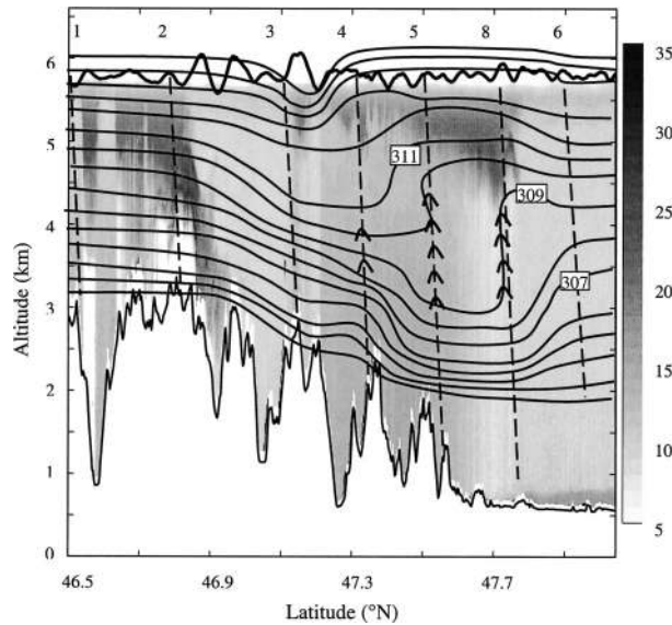
FIG. 4. The SABL backscatter coefficient (in grayscale), vertical displacement (thick solid curve between 5–6 km), and potential temperature contours (solid, interval = 1 K) along the first transverse. The vertical displacement is computed from the flight-level winds using Eq. (1). The potential temperature is derived from GPS dropsondes (see text for details). The dashed lines are GPS dropsonde trajectories and the dropsondes are numbered sequentially in time. The symbol \wedge indicates turbulent regions above the boundary layer. The terrain along the flight track is shown along the bottom.
