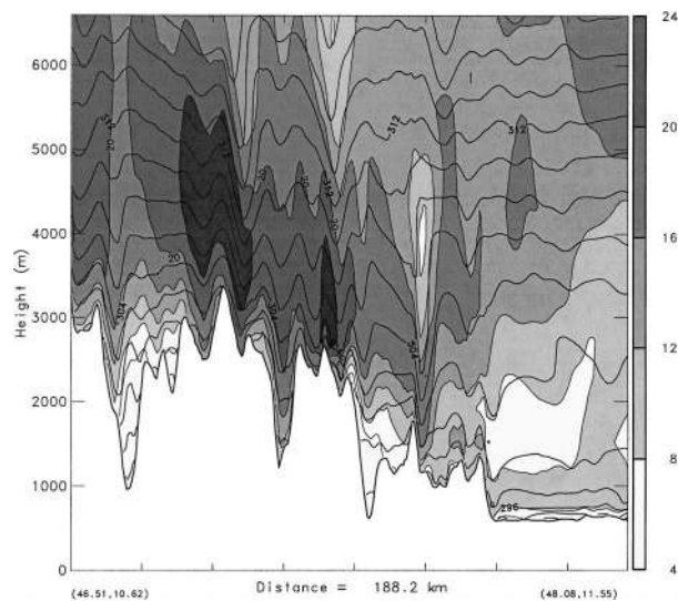
FIG. 16. Same as Fig. 14, except for a section corresponding to the second transverse and valid at 0730 UTC 21 Oct 1999.
