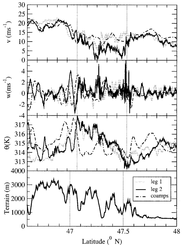
FIG. 8. The plot of two wind components (i.e., v and w ), and potential temperature (K) vs the latitude ( ^{\circ}\text{N} ) from flight-level data and COAMPS. The gray curves are for the first transverse and the dark curves for the second. Dotted-dashed curves are derived from the COAMPS simulation. The corresponding terrain (m) along the first transverse is included for reference.
