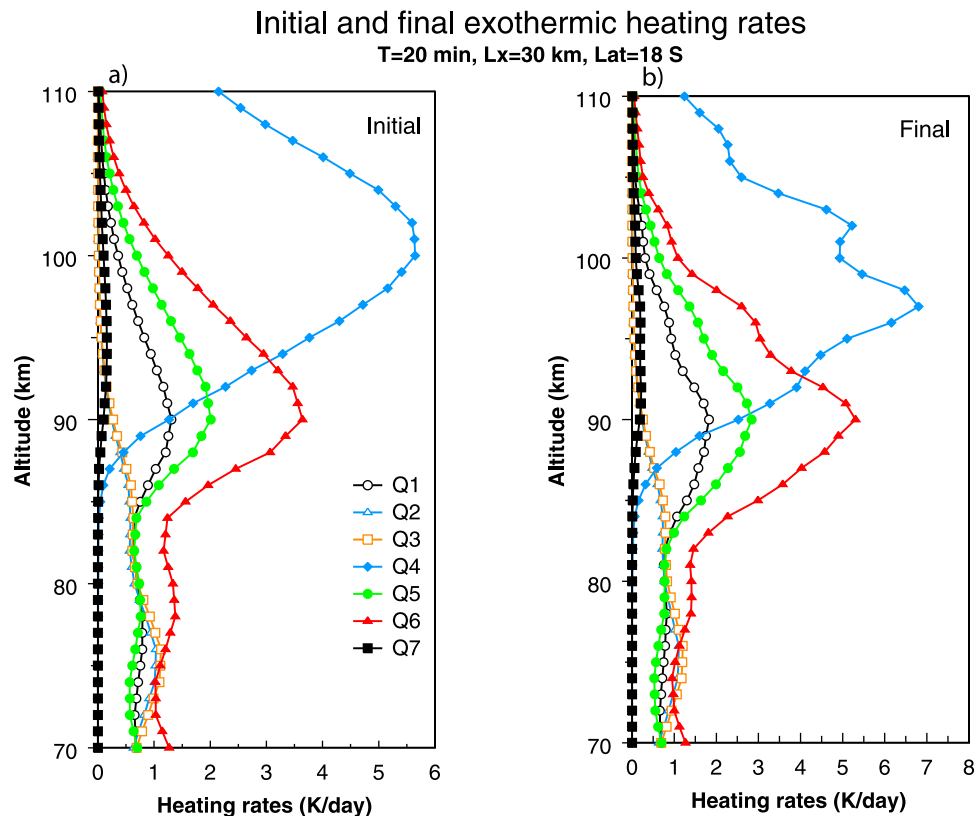
Figure 4. (a) Initial and (b) final exothermic heating rates Q_1 through Q_7 for 18^\circ\text{S} . The black curve with open circles denotes Q_1 , the blue curve with open triangles denotes Q_2 , the orange curve with open squares denotes Q_3 , the blue curve with solid diamonds denotes Q_4 , the green curve with solid circles denotes Q_5 , the red curve with solid triangles denotes Q_6 , and, finally, the black curve with solid squares denotes Q_7 . Q_4 and Q_6 are the major heating rates. The initial heating rate Q_4 peaks at 101 km altitude with a peak value of 5.64 \text{ K d}^{-1} while the final Q_4 peaks at 97 km with a value of 6.8 \text{ K d}^{-1} .
