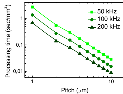
Fig. 5 Processing time of 1 \text{mm}^2 area versus pitch at different laser repetition rates: (■) - 50 kHz; (●) - 100 kHz; (▲) - 200 kHz.
