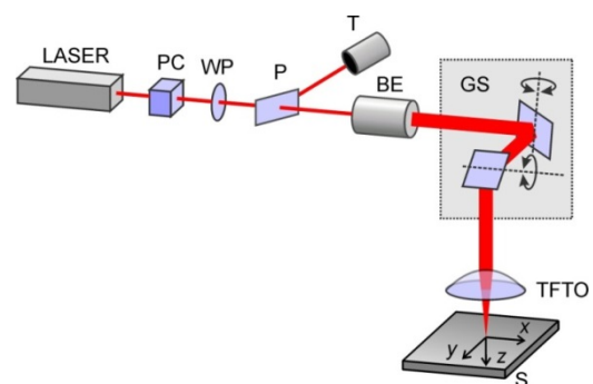
Fig. 1 Principal scheme of experimental setup: LASER - picosecond laser, PC - Pockels cell, WP - half wavelength wave plate, P - polarizer, T - trap, BE - beam expander, GS - galvanometer scanner, TFTO - telecentric-f-theta objective, S - sample, xy - denotes beam positioning directions, z - beam propagation direction.
