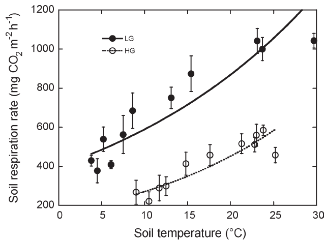
Fig. 3. Measured diurnal soil CO 2 flux vs. soil temperature. The equations for the predicted model are soil CO 2 flux ( y ) = 420 exp (0.039 soil temperature), r = 0.913 , p < 0.001 for the LG site and CO 2 flux ( y ) = 163 exp (0.051 soil temperature), r = 0.897 , p < 0.001 for the HG site. Vertical bars indicate the standard error of the measurement mean ( n = 3 ) for each time.
