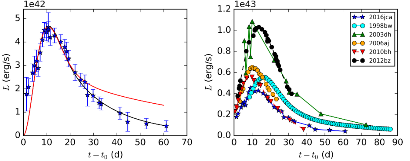
Fig. 12. The radioactive heating model (Arnett 1982) fit to the bolometric ( griz ) LC of SN 2016jca. Left: Two versions of the model have been fit to the data, one that assumes full trapping of \gamma -rays (red), and one which allows \gamma -ray leakage (black). It is seen that the latter model better fits the data. Both models require a nickel mass of M_{\text{Ni}} = 0.22 M_{\odot} , an ejecta mass of M_{\text{ej}} = 5.8 M_{\odot} , and for a peak photospheric velocity of v_{\text{ph}} = 29\,700 \pm 1\,500 \text{ km s}^{-1} , a kinetic energy of E_{\text{K}} = 5.1 \pm 0.8 \times 10^{52} \text{ erg} . Both models assume a grey optical opacity of \kappa = 0.07 \text{ cm}^2 \text{ g}^{-1} . In the latter model, we find a \gamma -ray opacity of \kappa_{\gamma} = 0.034 \text{ cm}^2 \text{ g}^{-1} . Right: Comparison of the optical bolometric LCs of a small sample of GRB-SNe: SN 1998bw ( BVRI ), SN 2003dh ( UBVR ), SN 2006aj ( BVRI ), SN 2010bh ( griz ) and SN 2012bz ( griz ).
