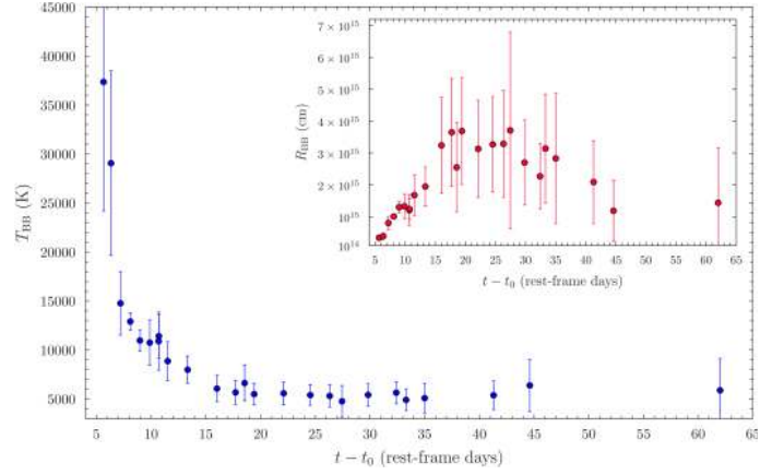
Fig. 11. Evolution of the BB colour temperature ( T_{\text{BB}} , blue) and radius (inset, red, R_{\text{BB}} ). The colour temperature corresponds to filters griz .
