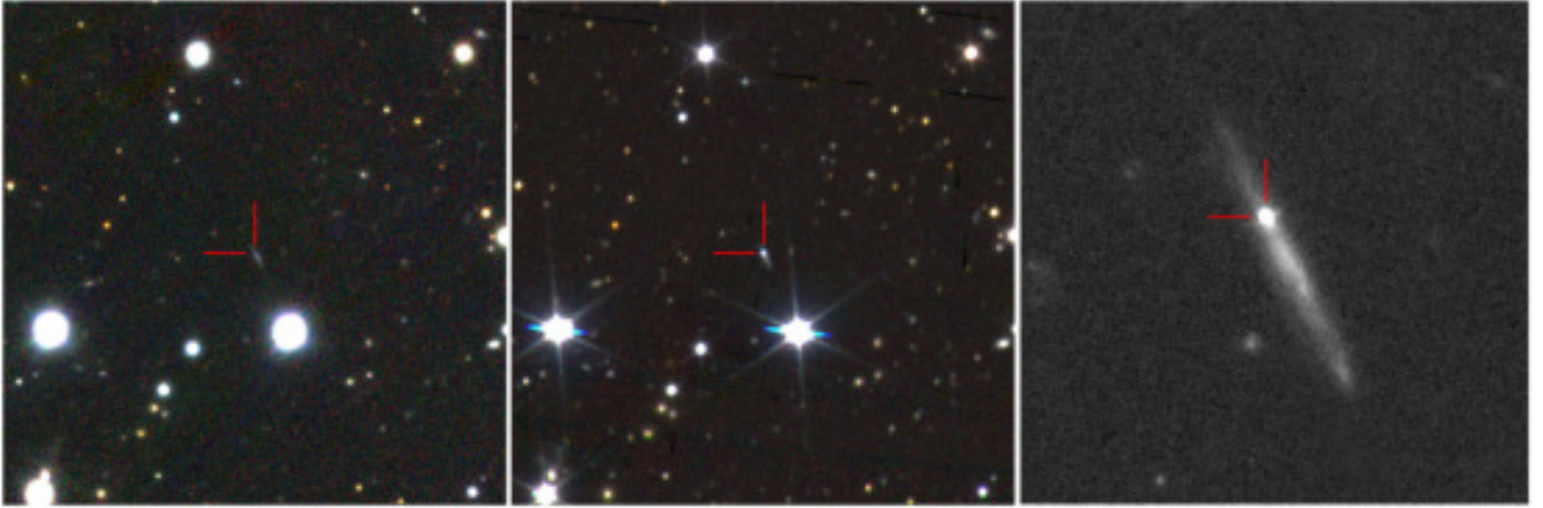
Fig. 1. Left: RGB composite Pan-STARRS1 pre-imaging of the host galaxy. Centre: a GTC image (RGB) showing the supernova starting to emerge on the 27 th of December, 2016. Right: HST WFC/UVIS F200LP image of the host galaxy and optical transient from the January 16 th , 2017.
