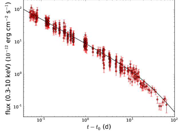
Fig. 3. The Swift -XRT LC of GRB 161219B / SN 2016jca (orbit 1 was omitted – see the main text for more details). A broken power-law was fit to the data, with the best-fitting parameters being: \alpha_1 = 0.79 \pm 0.02 , \alpha_2 = 1.93 \pm 0.28 , and the time the LC breaks between \alpha_1 and \alpha_2 being 38.0 \pm 7.3 days ( \chi^2/\text{dof} = 389.2/348 ).
