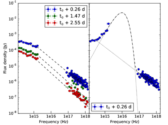
Fig. 4. NIR to X-ray SED of GRB 161219B at t - t_0 = 0.26, 1.47 and 2.55 days. Left: The best-fitting model consisting of a broken power-law and MW extinction curve. For all three epochs, we find: \beta_{opt} \approx 0.45 , \beta_X \approx 0.95 and a break frequency of \nu_B \approx 1.7 - 1.8 \times 10^{15} Hz. The local reddening is low ( E(B - V) \approx 0.02 mag). Right: To the SED at +0.26 days, we fit an extinguished broken power-law with an additional blackbody component. At this early epoch ( \approx +5.4 hours, rest-frame), the BB component is very hot ( T_{BB} \approx 0.16 \times 10^6 K) and it contributes \approx 68\% of the total recorded flux. (Note that the BB fit implies a larger local reddening than the BPL fits – see the main text for further discussion).
