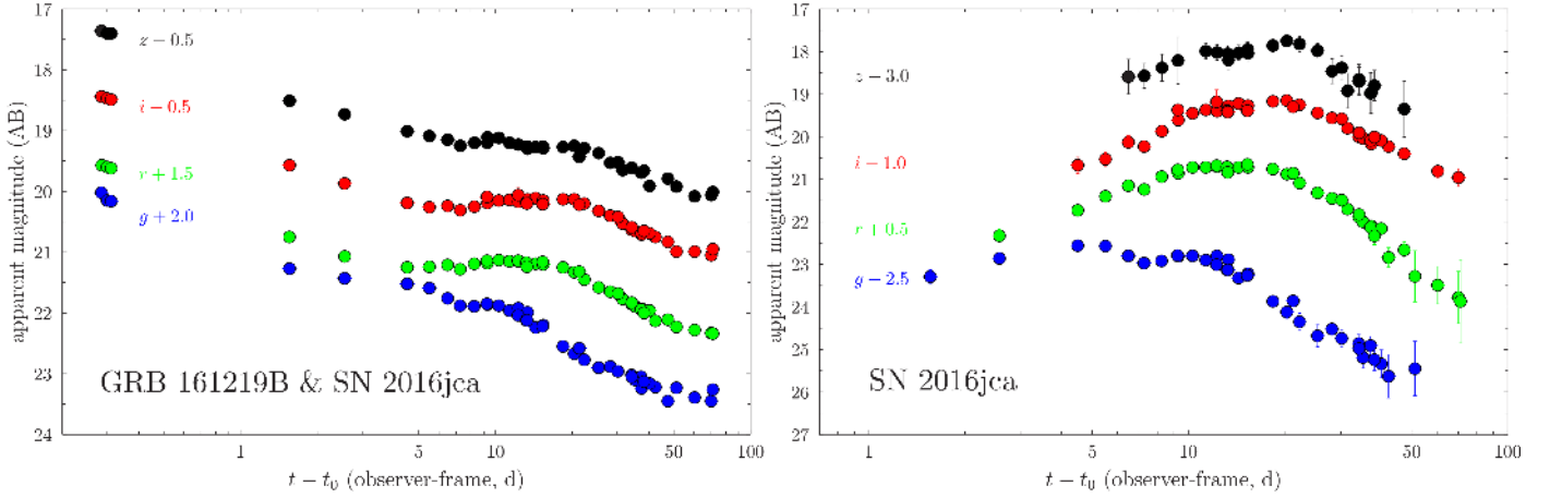
Fig. 5. Observer-frame optical ( griz ) LCs of GRB 161219B / SN 2016jca. Left: LCs of the AG, SN and underlying host, which are uncorrected for extinction. The typical evolution from the AG-dominated to the SN-dominated phase is seen in all optical filters. Right: Host- and AG-subtracted LCs of SN 2016jca. A pre-maximum bump is seen in the g -band, which peaks around \approx 5 - 6 days. This bump is conspicuously absent in the other filters, and the origin of this flux excess is discussed in Sect. 8. In contrast, the potential bump seen in the z -band LC around 10 days is not real, but arises from instrumental defects.
