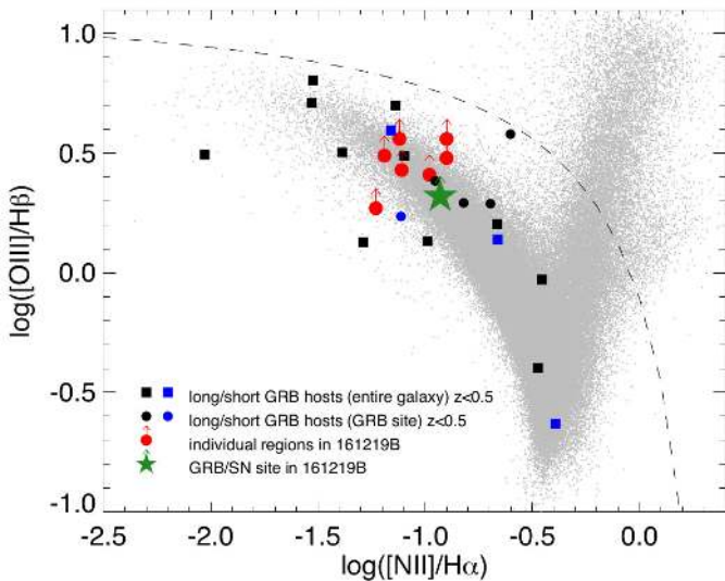
Fig. 17. BPT diagram showing the different regions in the host of GRB 161219B, where the GRB site is highlighted by the green star. Values presented here are only lower limits as H\beta could not be measured due to its location on top of an atmospheric emission line. Grey dots are galaxies from SDSS (DR9), while the squares and dots are other GRB hosts/GRB sites (the latter for cases of resolved galaxies) at z < 0.5 . The dashed line marks the dividing line between SF regions and those dominated by AGN activity. Data are taken from Christensen et al. (2008); Berger (2009); Han et al. (2010); Levesque et al. (2010); Perley et al. (2012); Thöne et al. (2014); de Ugarte Postigo et al. (2014b); Schulze et al. (2014); Stanway et al. (2015); Krühler et al. (2015).
