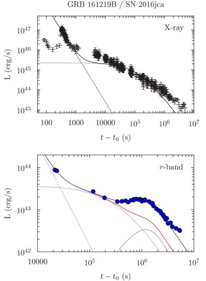
Fig. 13. Magnetar model from Cano et al. (2016b) fit to the X-ray (Top) and r -band (Bottom) luminosity LCs. Times are shown in the rest-frame. Top: The sum of the SPL (dot-dashed line) and magnetar-powered AG (dotted line) phases is shown as the solid black line. Visual inspection shows that the model fails to reproduce the decay seen in the observations at t - t_0 > 3 \times 10^5 \text{ s} . The best-fitting model gives B_0 = 1.0 \times 10^{15} \text{ G} , and P_0 = 8.1 \text{ ms} . Bottom: The sum of the SPL (dot-dashed line), magnetar-powered AG (dotted line) and magnetar-powered SN (dashed line) phases is shown as the solid red line. The solid blue line includes an additional multiplicative factor ( \Psi ) to get the magnetar-powered SN to match the observations. The best-fitting model gives B_0 = 2.4 \times 10^{15} \text{ G} , and P_0 = 35.2 \text{ ms} , which are clearly discrepant with those determined from the X-ray. In addition, we found a diffusion time scale of t_{\text{diff}} = 9.43 \pm 0.10 \text{ days} , and \Psi = 4.2 \pm 0.1 . The conclusion is that the magnetar model cannot self-consistently explain the X-ray and optical observations of GRB 161219B/SN 2016jca. Even if SN 2016jca was powered in part by a magnetar central engine, an additional source of energy is needed to reproduce the observations, most likely a reservoir of radioactive nickel. The required nickel mass to get the model to match observations is M_{\text{Ni}} \sim 0.4 M_\odot .
