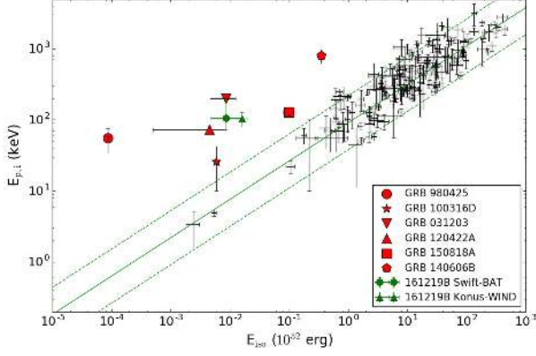
Fig. 2. The position of the intermediate-luminosity GRB 161219B in the E_{p,i} - E_{iso} (Amati) plane. Shown for comparison is the GRB sample presented in Amati et al. (2002) and (Cano et al. 2015), as well as other outliers of the Amati relation, including low-luminosity GRBs 980425, 031203 & 100316D, intermediate-luminosity GRB 150818A and high-luminosity GRBs 120422A & 140606B.
