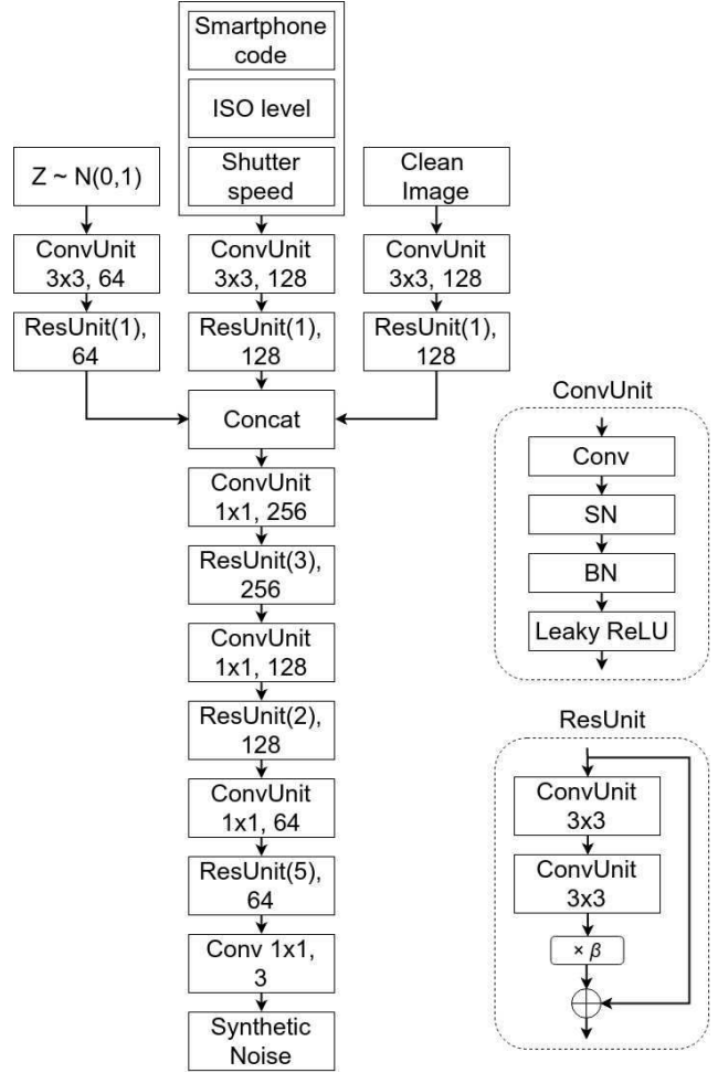
Figure 3: cERGAN generator.
